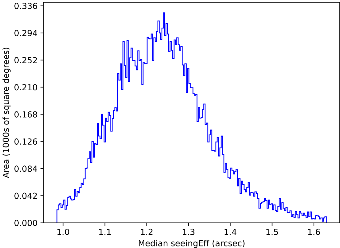
too_elab_r16_d2_gz_v3.4_10yrs All sky u band: Median seeingEff
