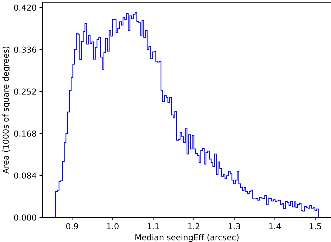
too_elab_r16_d2_gz_v3.4_10yrs All sky r band: Median seeingEff
