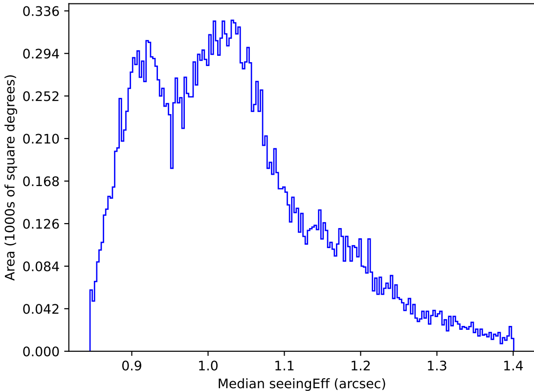
too_elab_r16_d2_gz_v3.4_10yrs All sky i band: Median seeingEff
