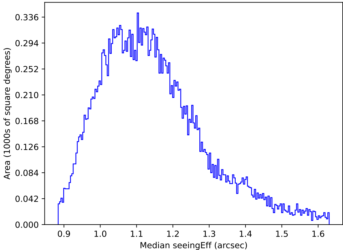
too_elab_r16_d2_gz_v3.4_10yrs All sky g band: Median seeingEff
