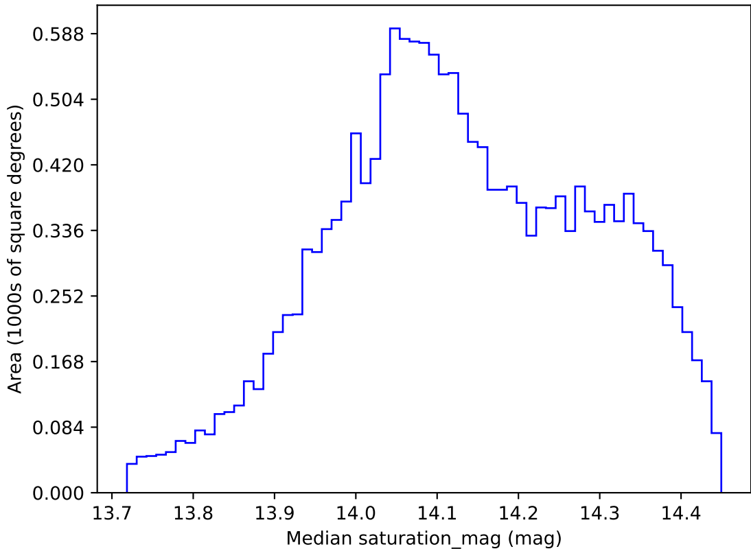
too_elab_r16_d2_gz_v3.4_10yrs WFD z band: Median saturation_mag
