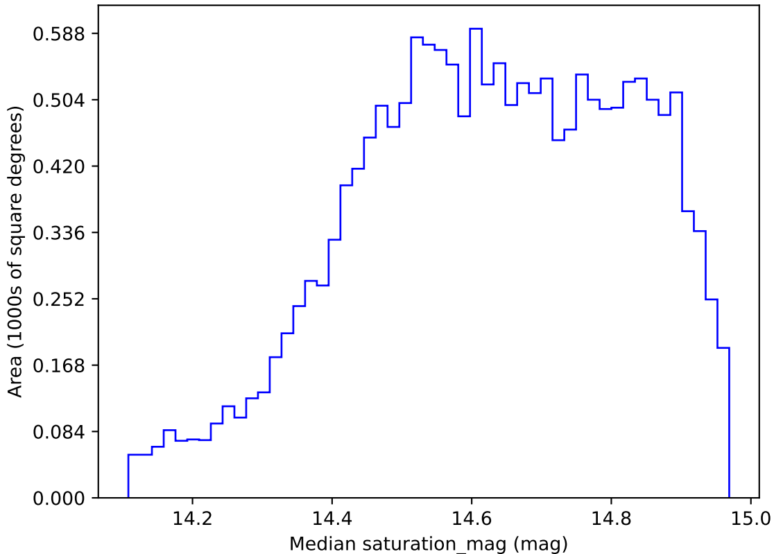
too_elab_r16_d2_gz_v3.4_10yrs WFD r band: Median saturation_mag
