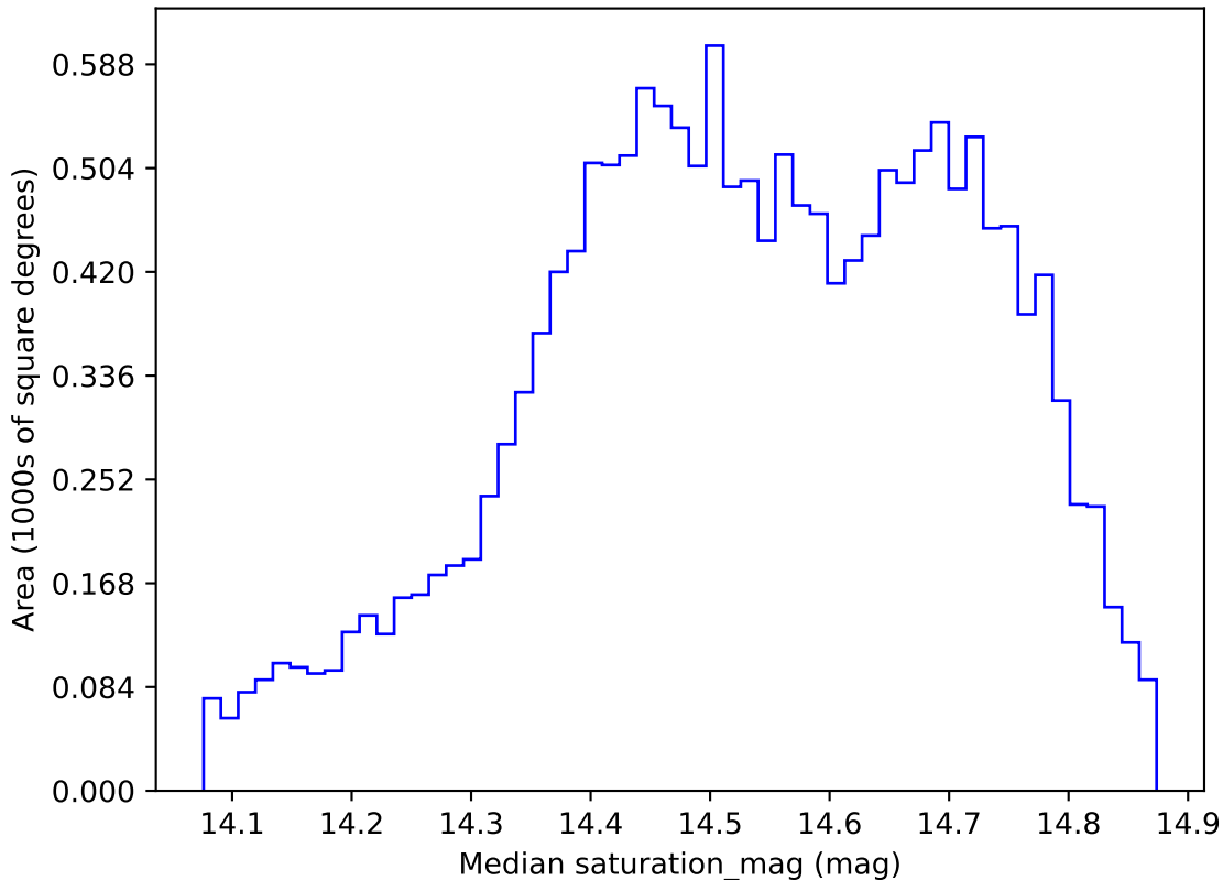
too_elab_r16_d2_gz_v3.4_10yrs WFD i band: Median saturation_mag
