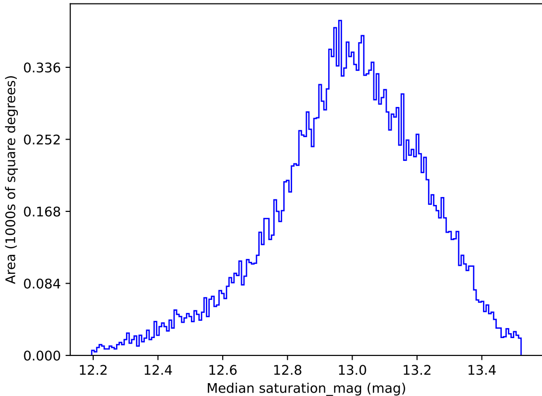
too_elab_r16_d2_gz_v3.4_10yrs All sky u band: Median saturation_mag
