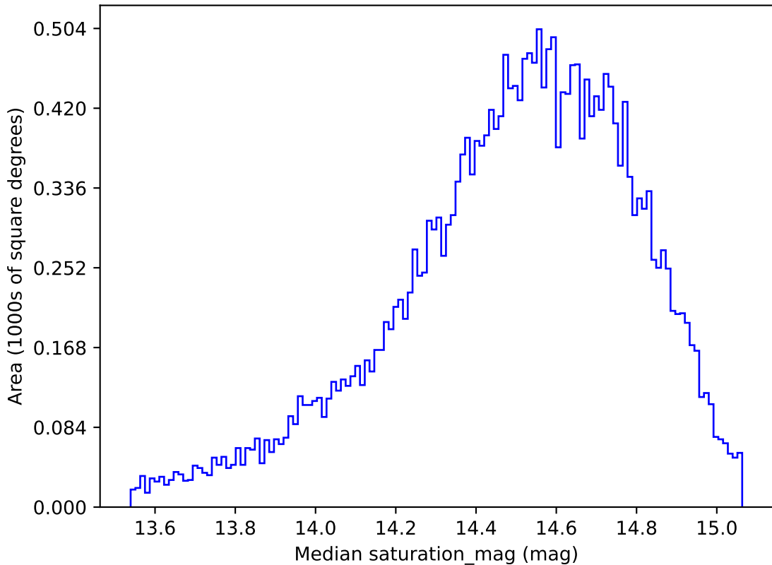
too_elab_r16_d2_gz_v3.4_10yrs All sky g band: Median saturation_mag
