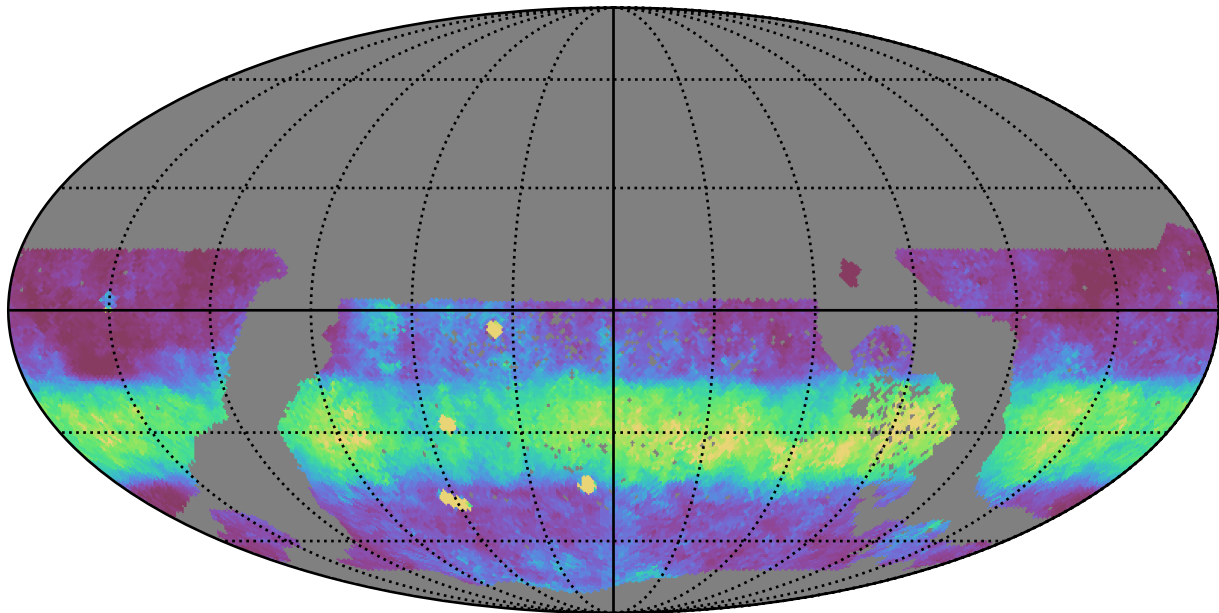
too_elab_r16_d2_gz_v3.4_10yrs WFD z band: Median normairmass
