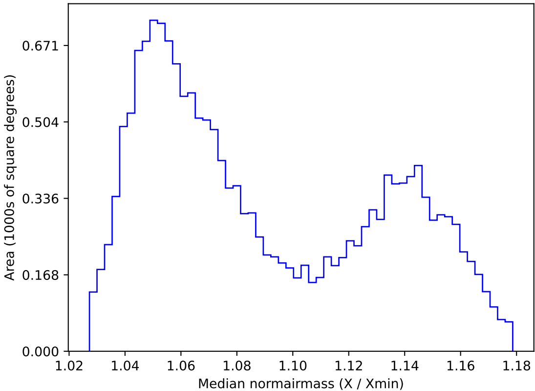
too_elab_r16_d2_gz_v3.4_10yrs WFD y band: Median normairmass
