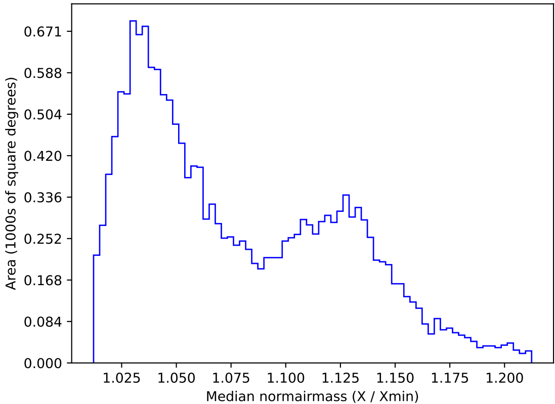
too_elab_r16_d2_gz_v3.4_10yrs WFD u band: Median normairmass
