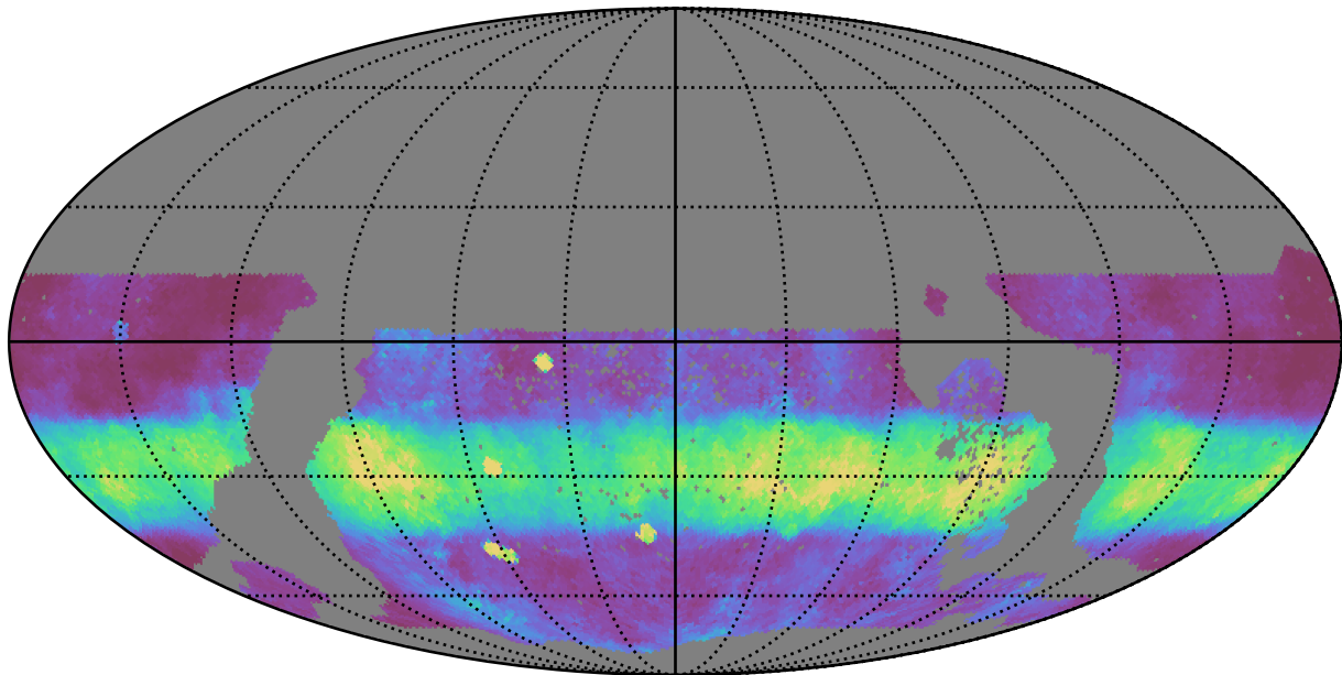
too_elab_r16_d2_gz_v3.4_10yrs WFD r band: Median normairmass
