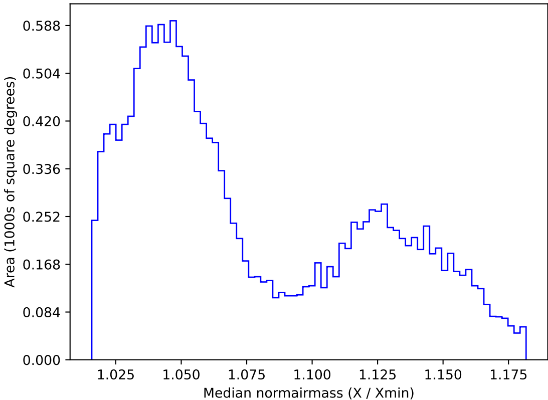
too_elab_r16_d2_gz_v3.4_10yrs WFD r band: Median normairmass
