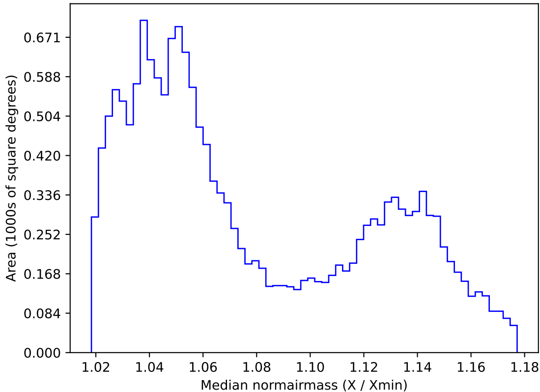
too_elab_r16_d2_gz_v3.4_10yrs WFD i band: Median normairmass
