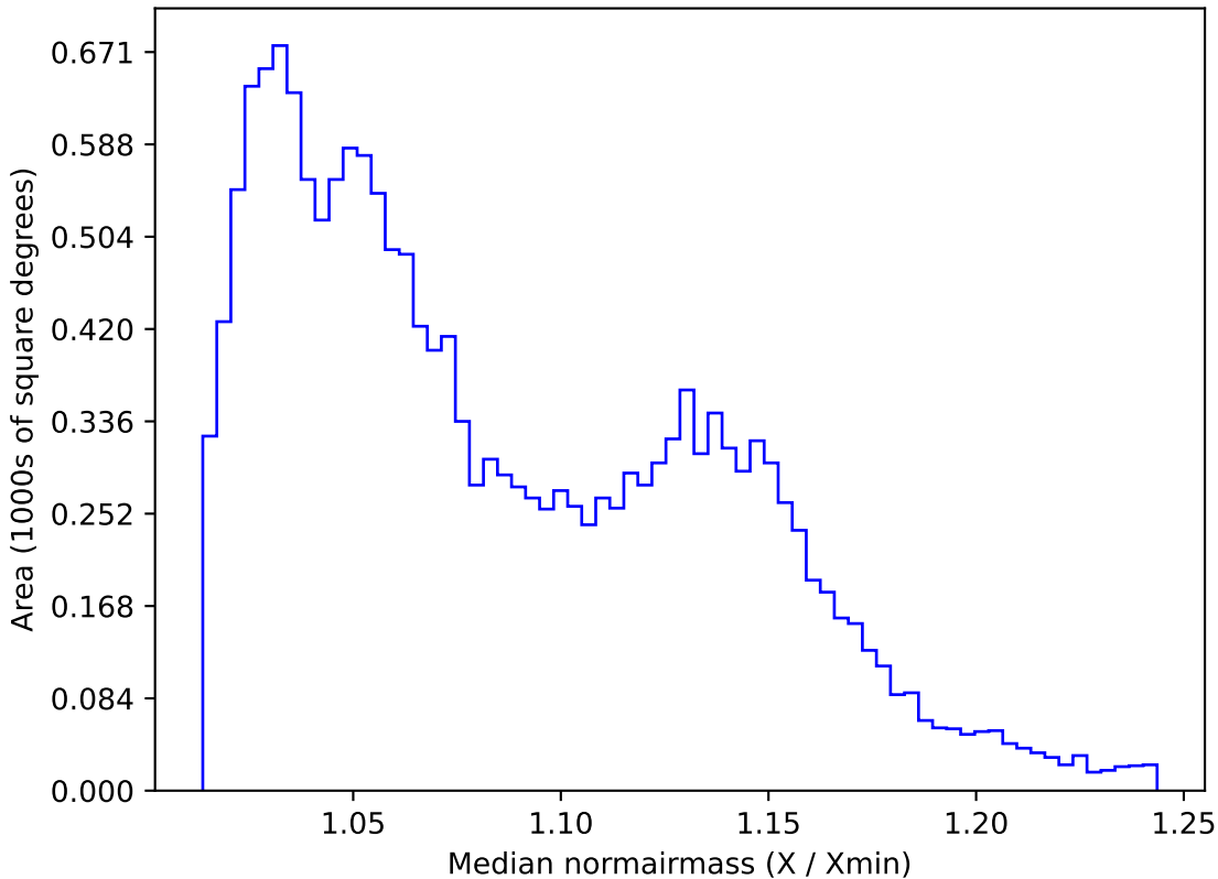
too_elab_r16_d2_gz_v3.4_10yrs WFD g band: Median normairmass
