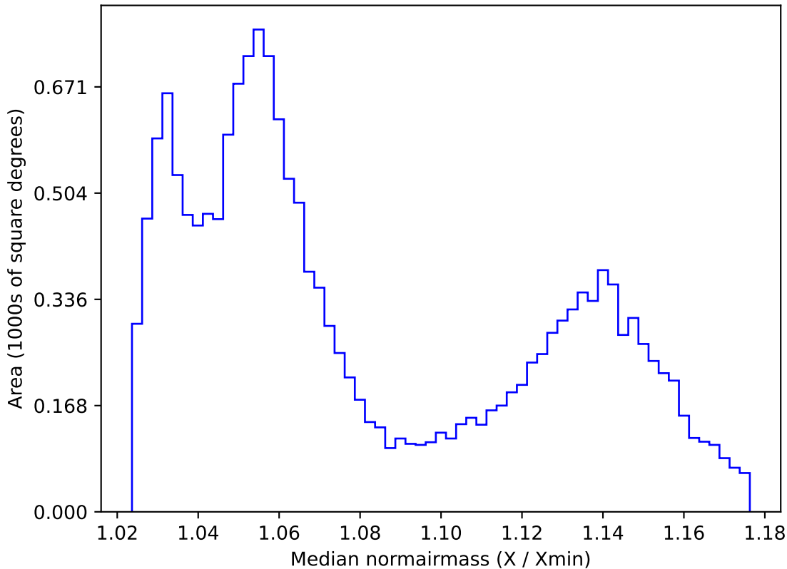
too_elab_r16_d2_gz_v3.4_10yrs WFD all bands: Median normairmass
