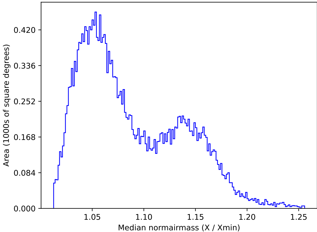
too_elab_r16_d2_gz_v3.4_10yrs All sky z band: Median normairmass
