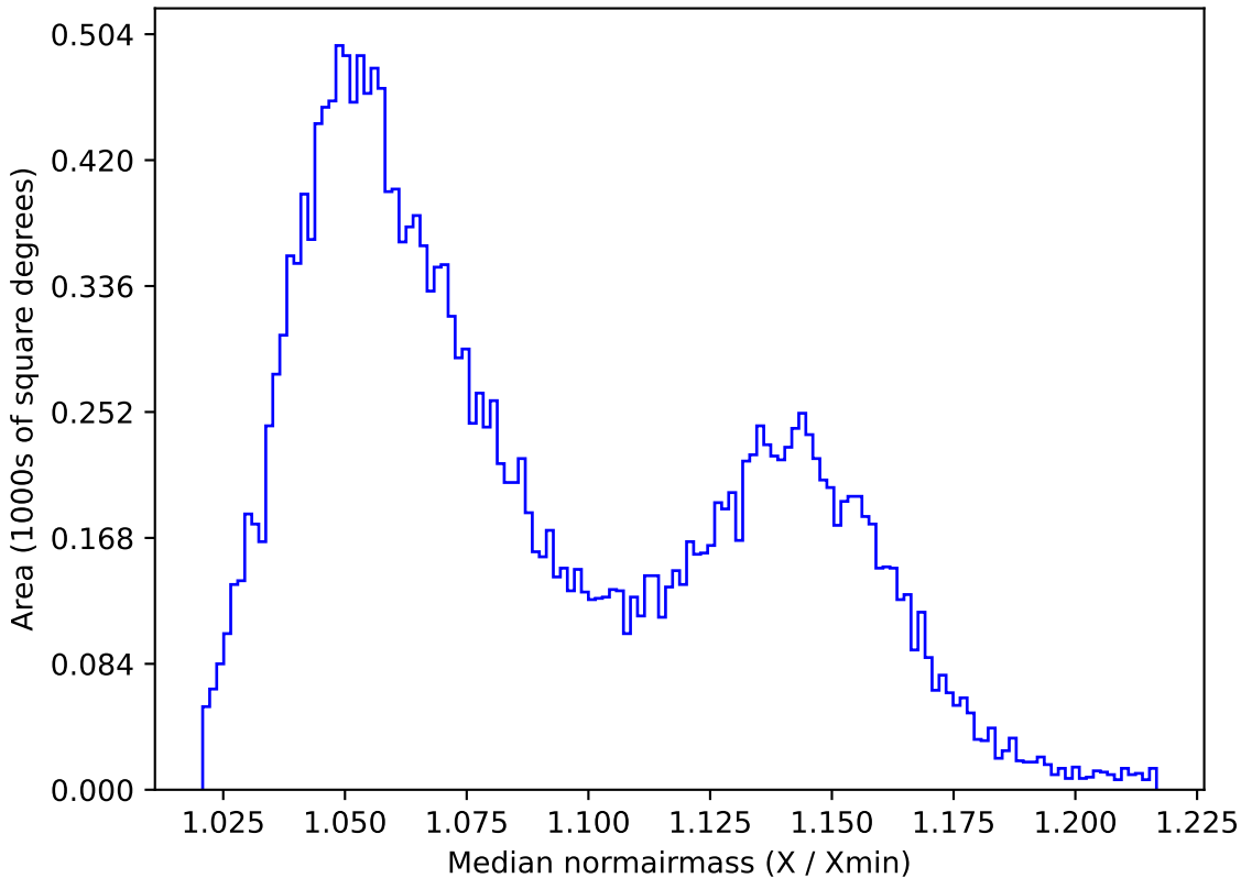
too_elab_r16_d2_gz_v3.4_10yrs All sky y band: Median normairmass
