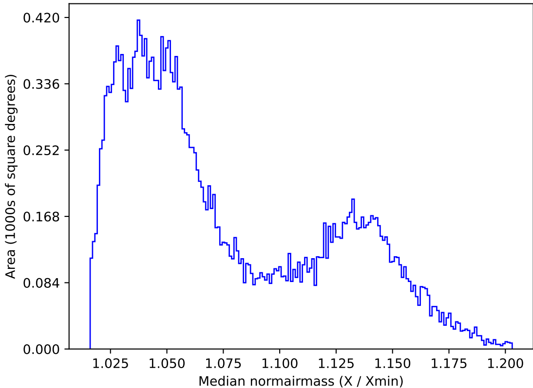
too_elab_r16_d2_gz_v3.4_10yrs All sky i band: Median normairmass
