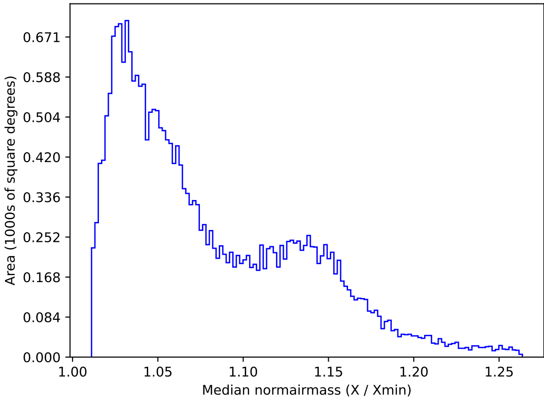
too_elab_r16_d2_gz_v3.4_10yrs All sky g band: Median normairmass
