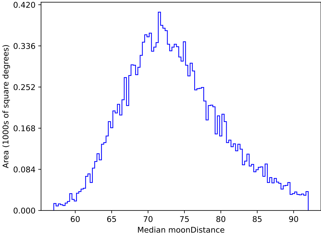
too_elab_r16_d2_gz_v3.4_10yrs WFD z band: Median moonDistance
