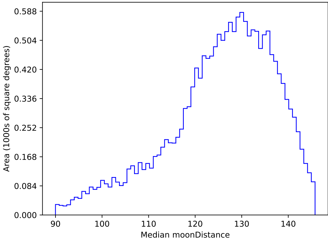
too_elab_r16_d2_gz_v3.4_10yrs WFD u band: Median moonDistance
