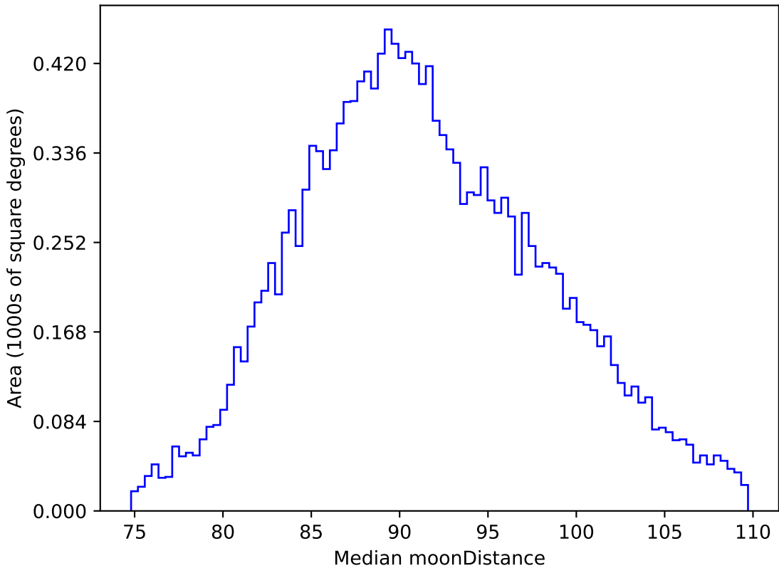
too_elab_r16_d2_gz_v3.4_10yrs WFD i band: Median moonDistance
