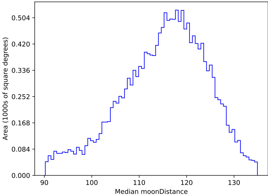
too_elab_r16_d2_gz_v3.4_10yrs WFD g band: Median moonDistance
