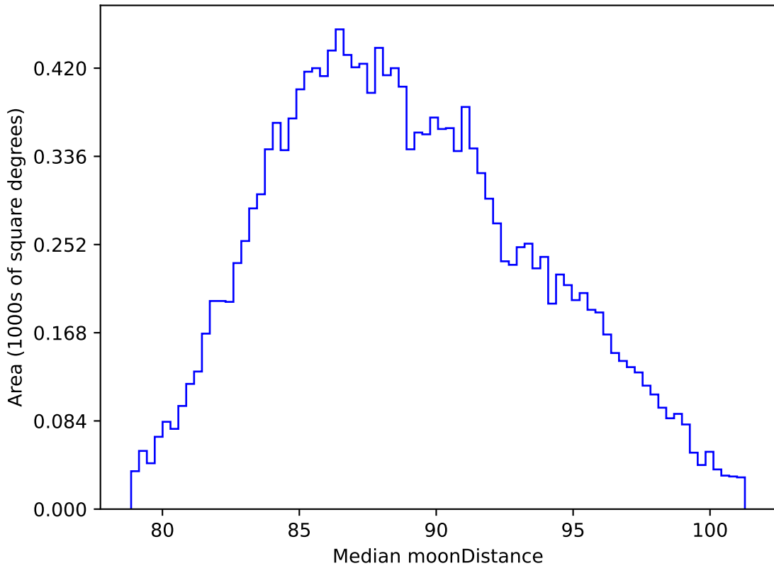
too_elab_r16_d2_gz_v3.4_10yrs WFD all bands: Median moonDistance
