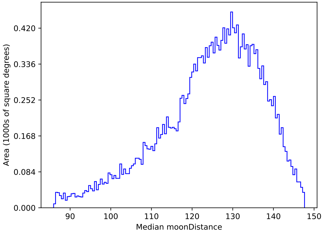
too_elab_r16_d2_gz_v3.4_10yrs All sky u band: Median moonDistance
