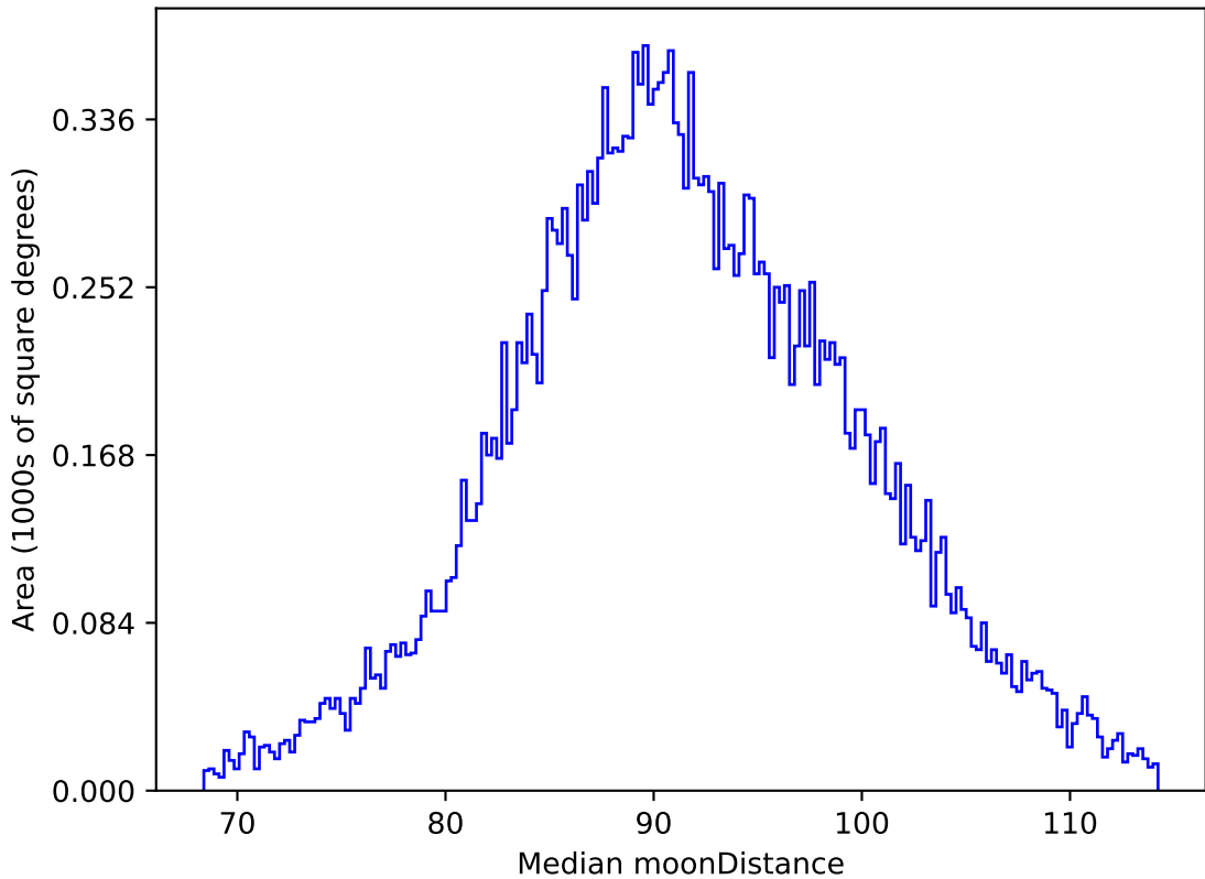
too_elab_r16_d2_gz_v3.4_10yrs All sky i band: Median moonDistance
