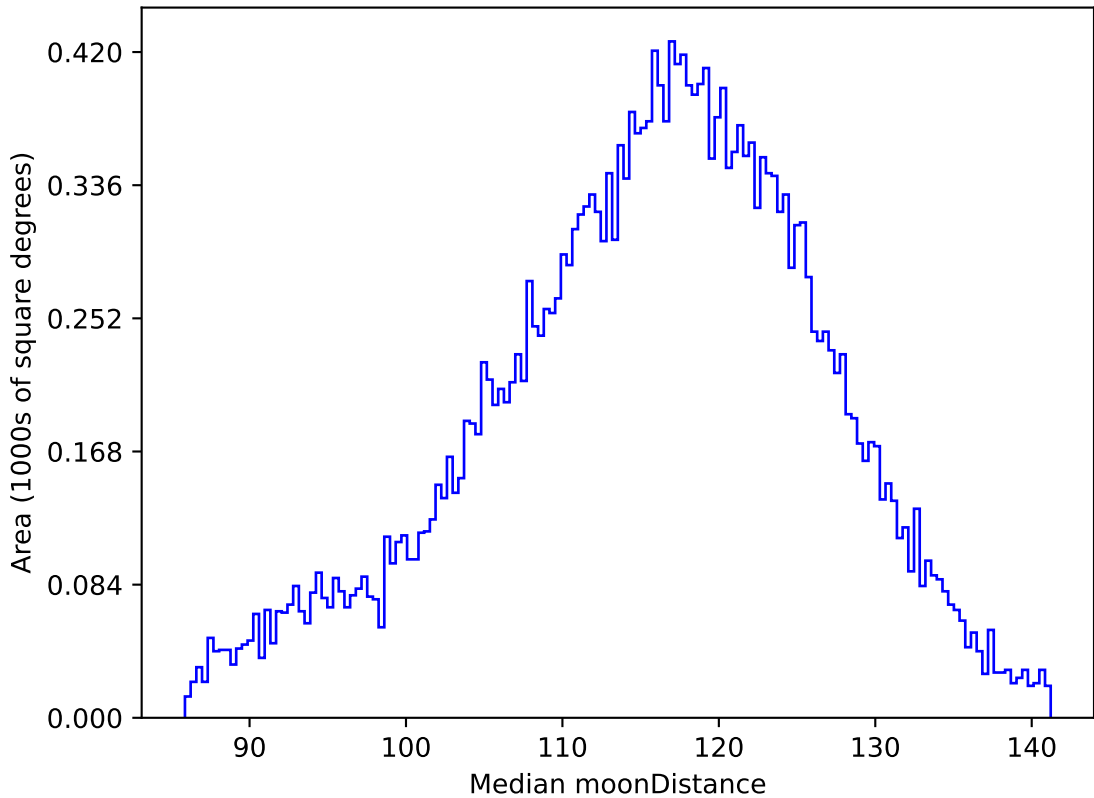
too_elab_r16_d2_gz_v3.4_10yrs All sky g band: Median moonDistance
