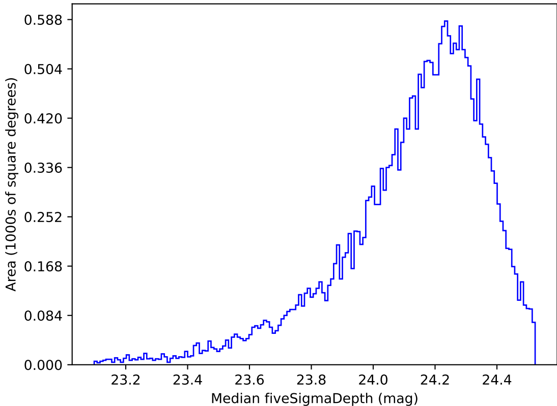
too_elab_r16_d2_gz_v3.4_10yrs Yr 1 r band: Median fiveSigmaDepth
