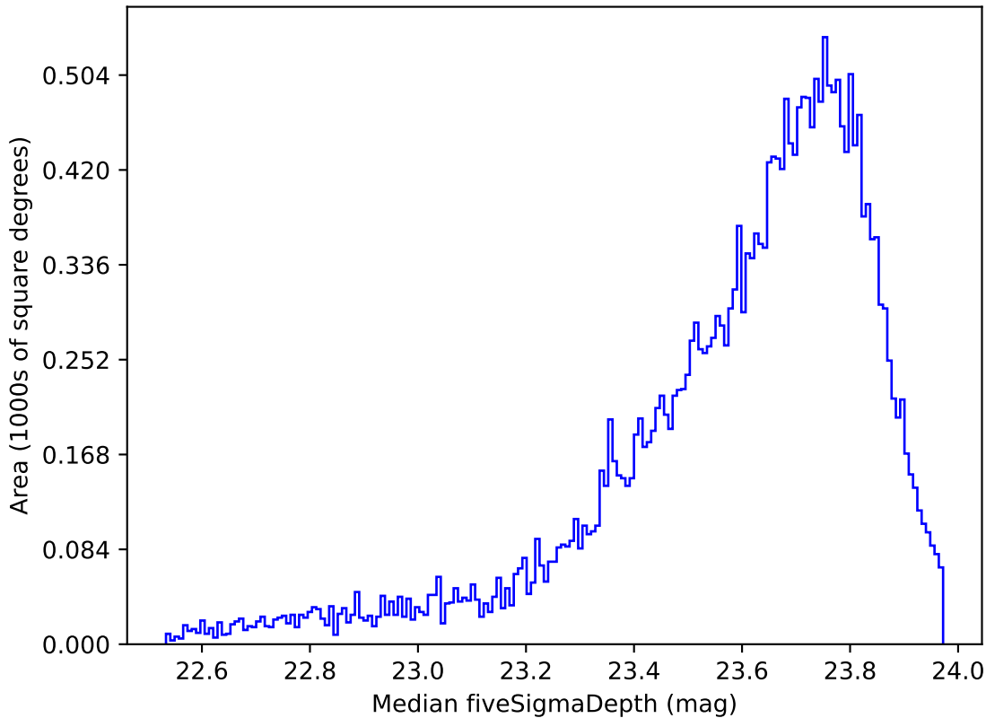
too_elab_r16_d2_gz_v3.4_10yrs Yr 1 i band: Median fiveSigmaDepth
