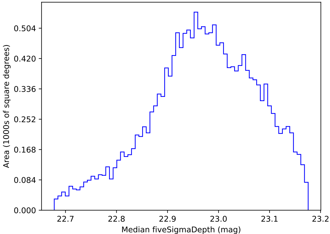
too_elab_r16_d2_gz_v3.4_10yrs WFD z band: Median fiveSigmaDepth
