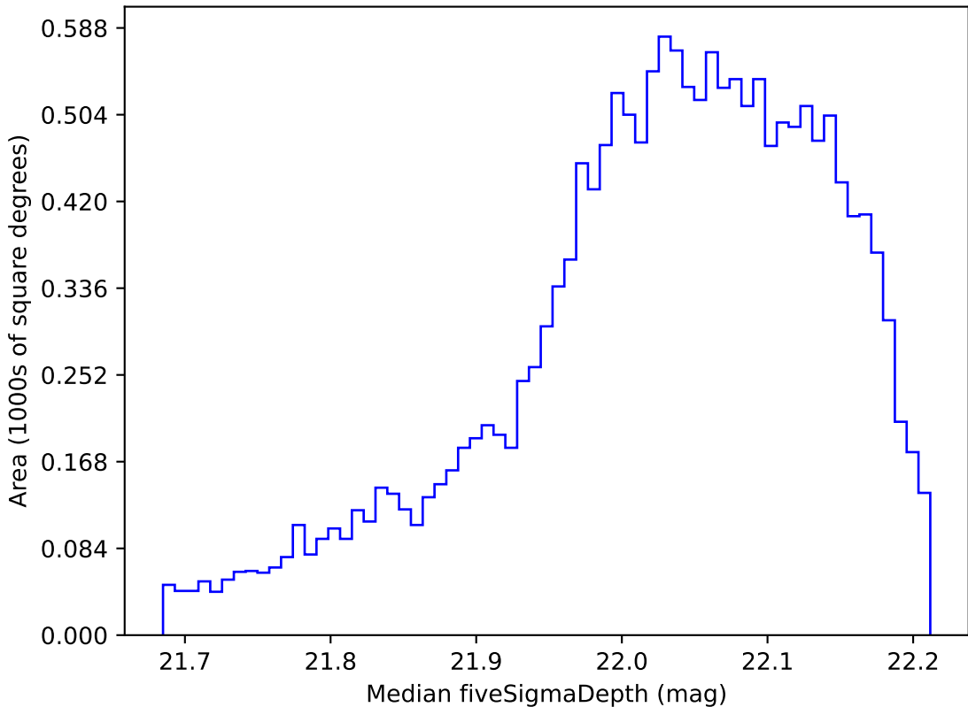
too_elab_r16_d2_gz_v3.4_10yrs WFD y band: Median fiveSigmaDepth
