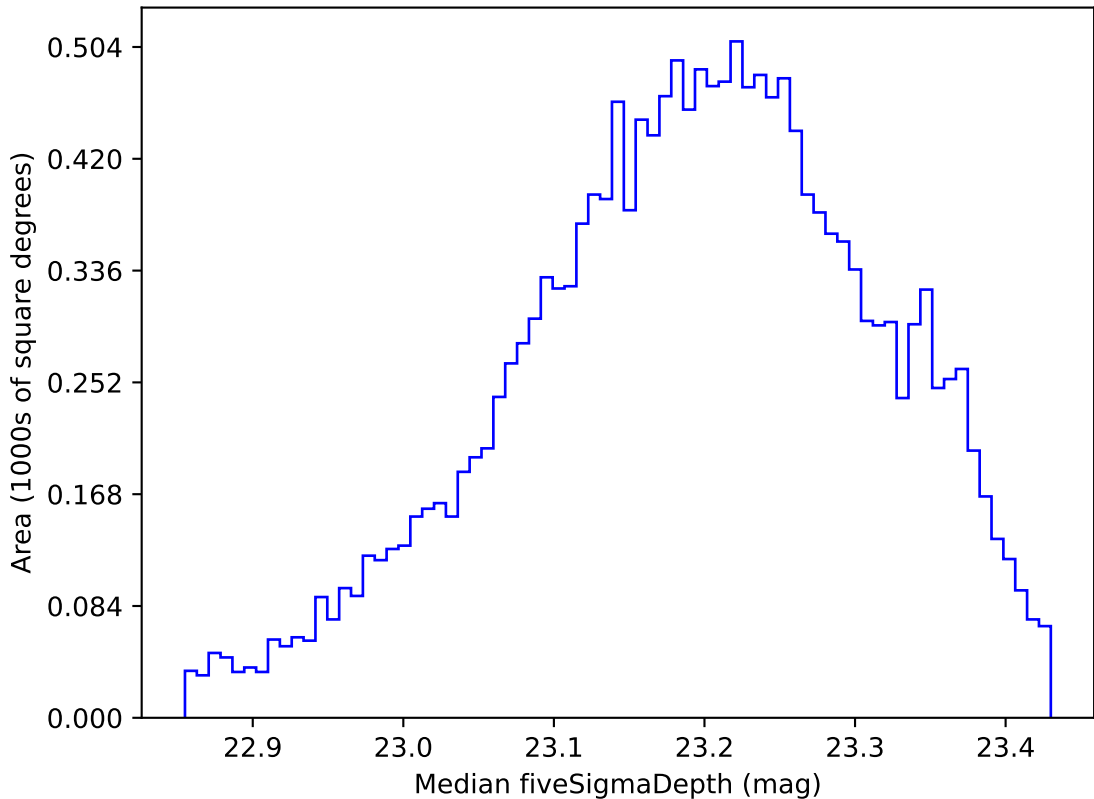
too_elab_r16_d2_gz_v3.4_10yrs WFD u band: Median fiveSigmaDepth
