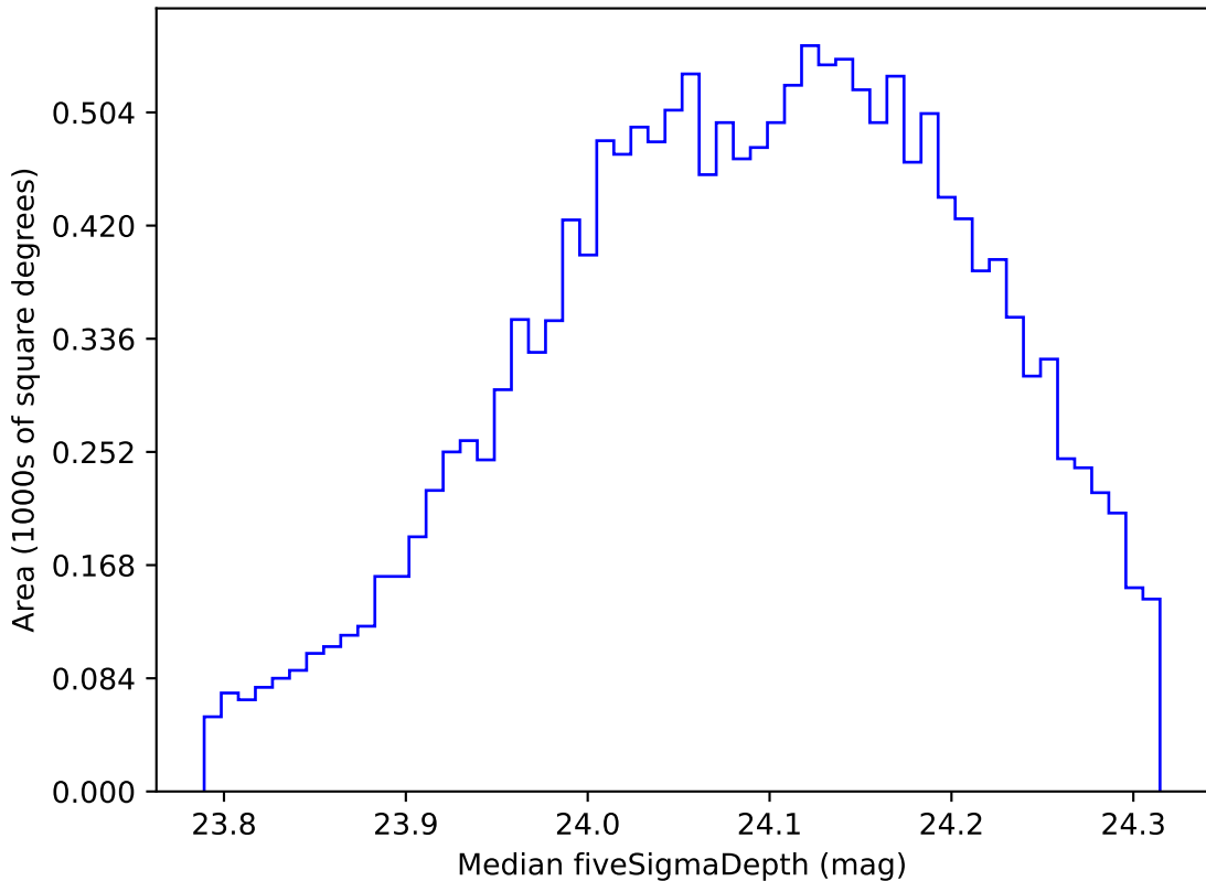
too_elab_r16_d2_gz_v3.4_10yrs WFD r band: Median fiveSigmaDepth
