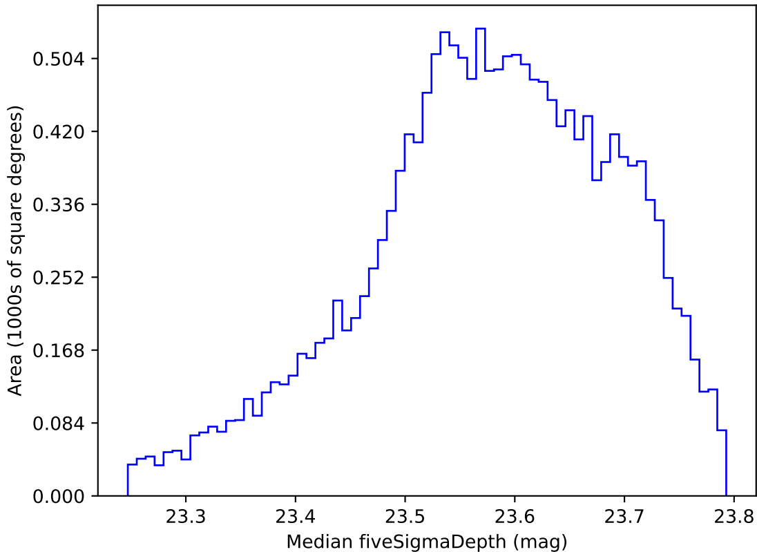
too_elab_r16_d2_gz_v3.4_10yrs WFD i band: Median fiveSigmaDepth
