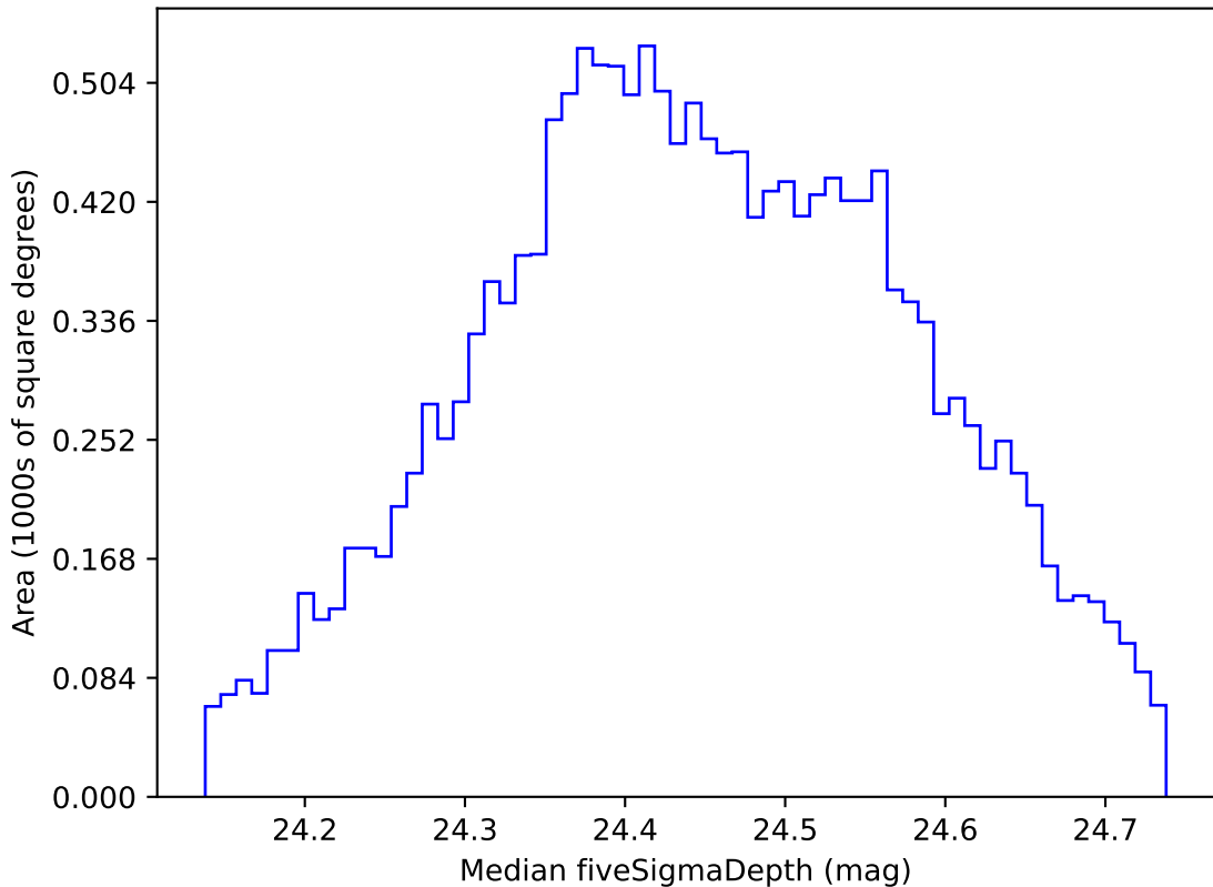
too_elab_r16_d2_gz_v3.4_10yrs WFD g band: Median fiveSigmaDepth
