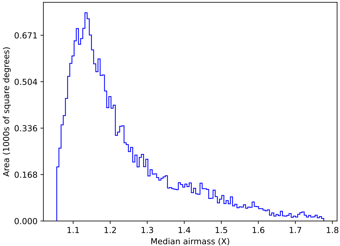
too_elab_r16_d2_gz_v3.4_10yrs Yr 1 u band: Median airmass
