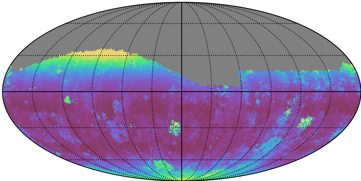
too_elab_r16_d2_gz_v3.4_10yrs Yr 1 g band: Median airmass
