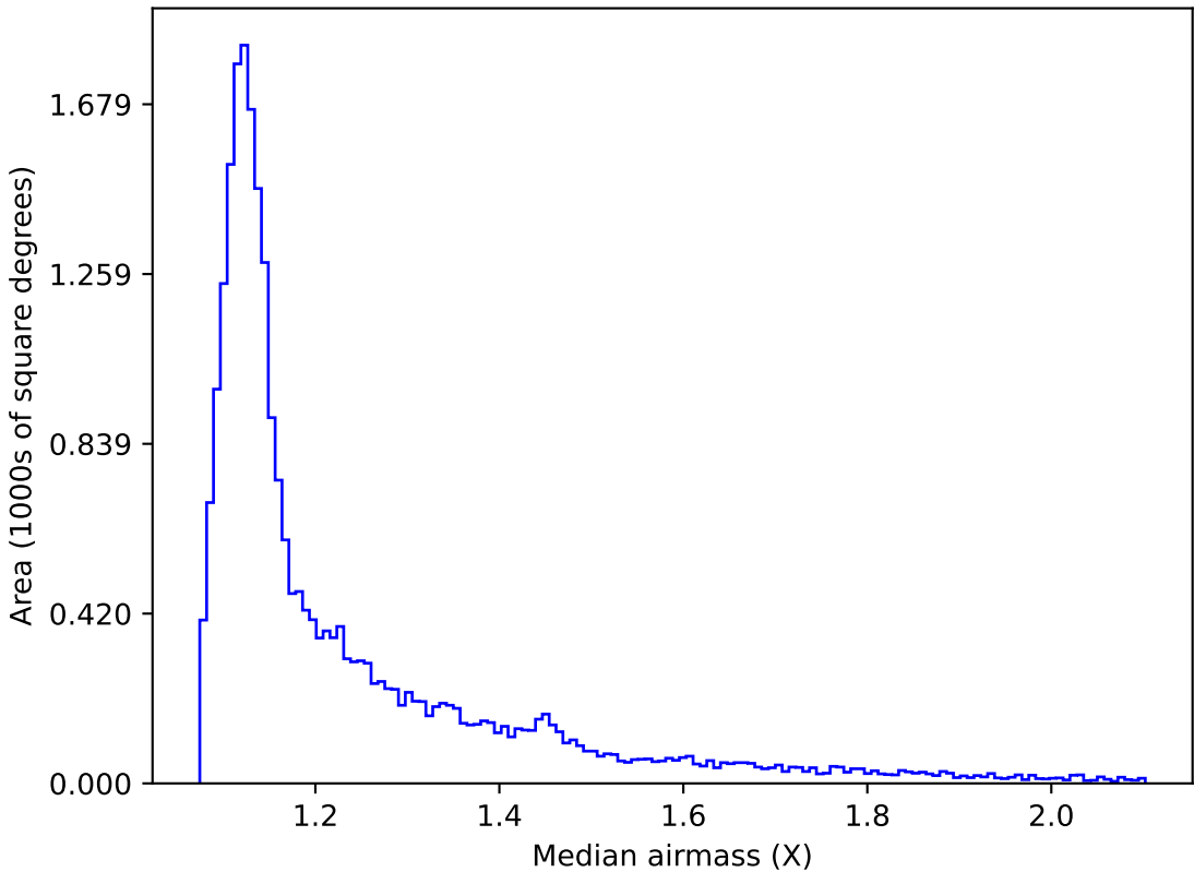
too_elab_r16_d2_gz_v3.4_10yrs Yr 1 all bands: Median airmass
