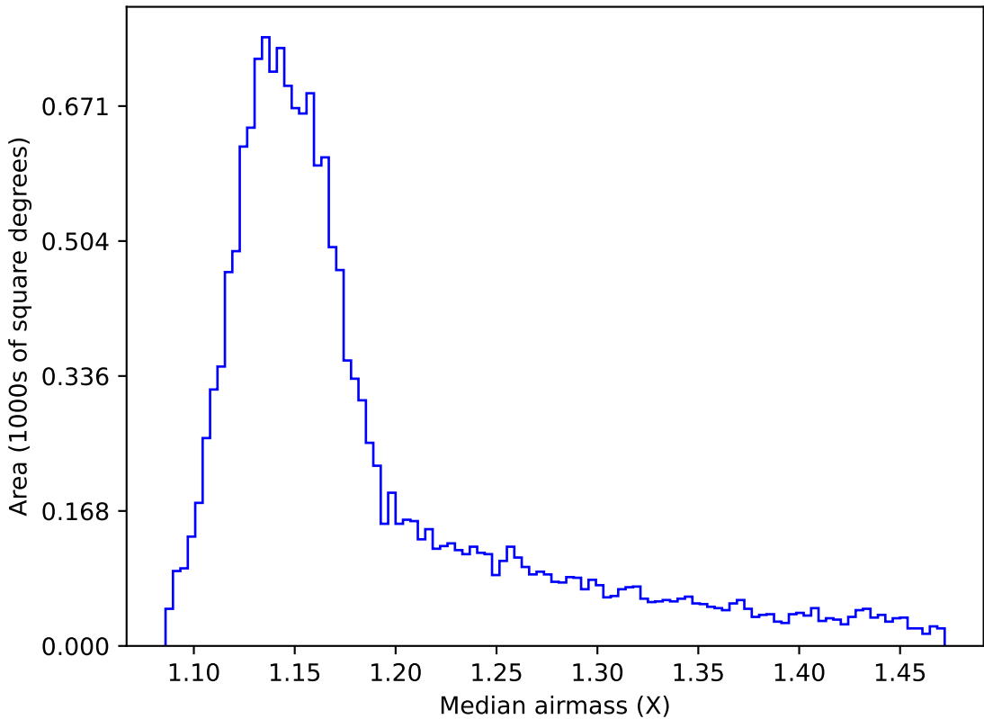
too_elab_r16_d2_gz_v3.4_10yrs WFD z band: Median airmass
