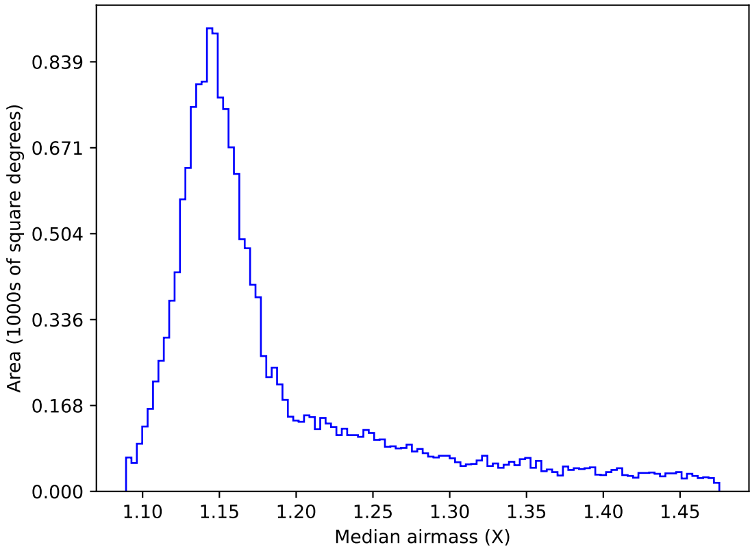
too_elab_r16_d2_gz_v3.4_10yrs WFD y band: Median airmass
