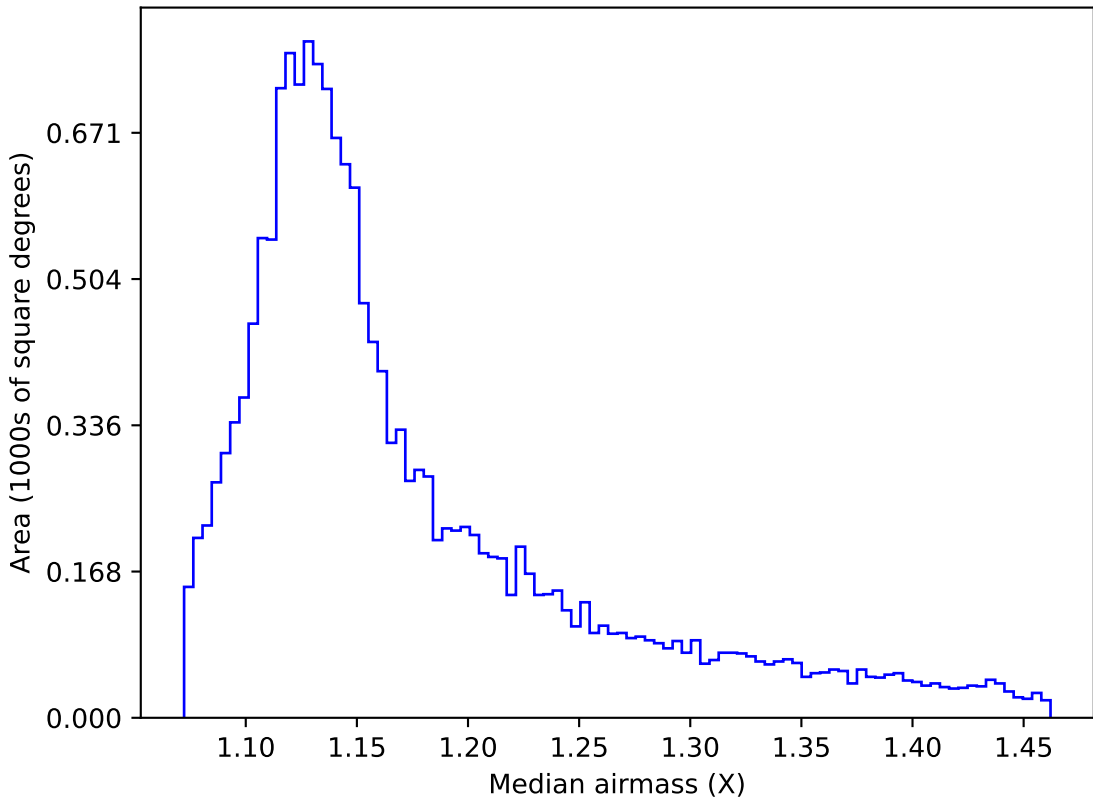
too_elab_r16_d2_gz_v3.4_10yrs WFD u band: Median airmass
