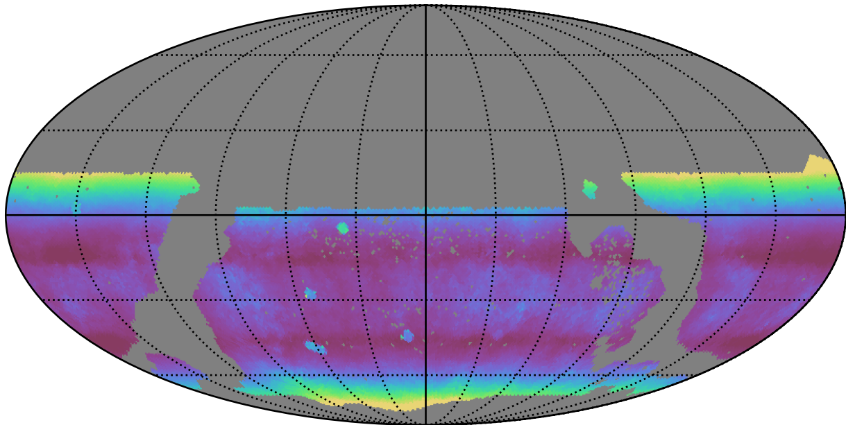
too_elab_r16_d2_gz_v3.4_10yrs WFD r band: Median airmass
