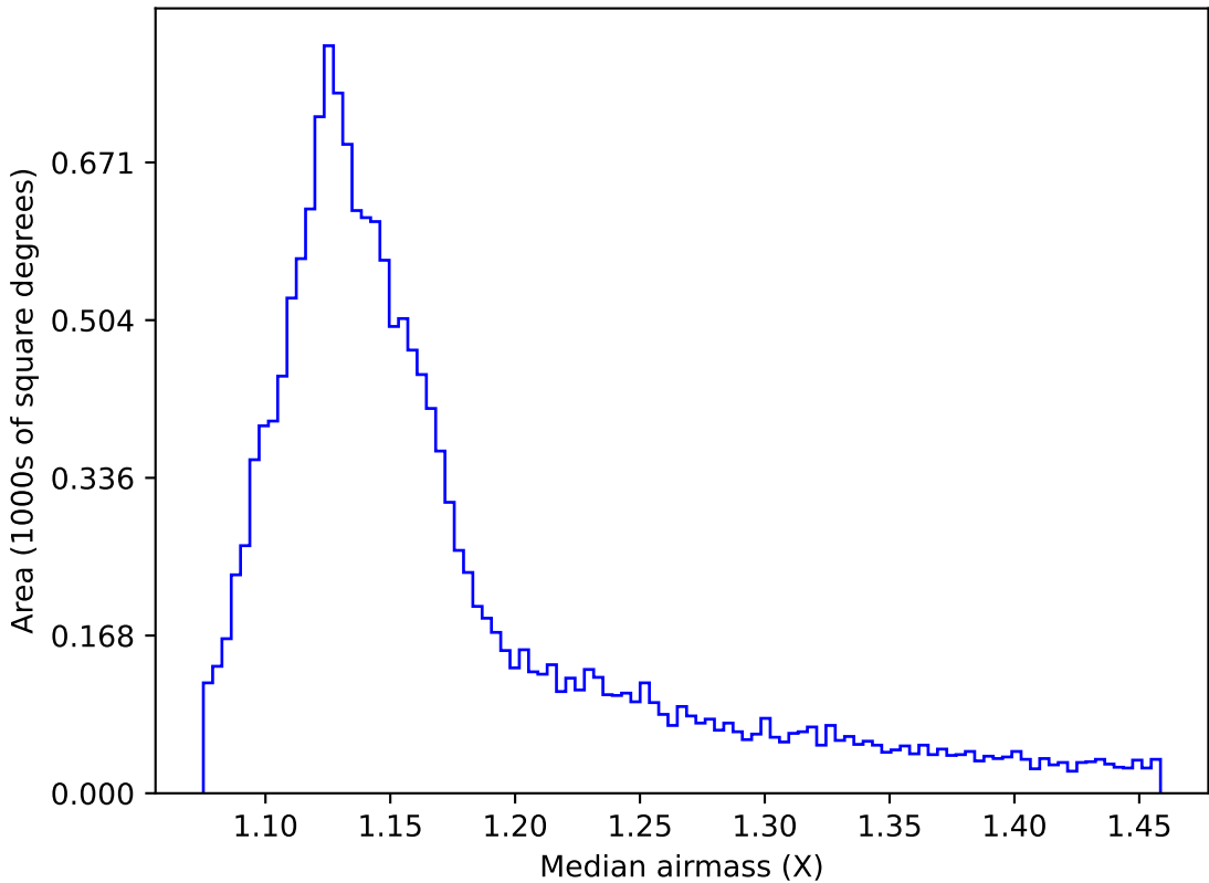
too_elab_r16_d2_gz_v3.4_10yrs WFD r band: Median airmass
