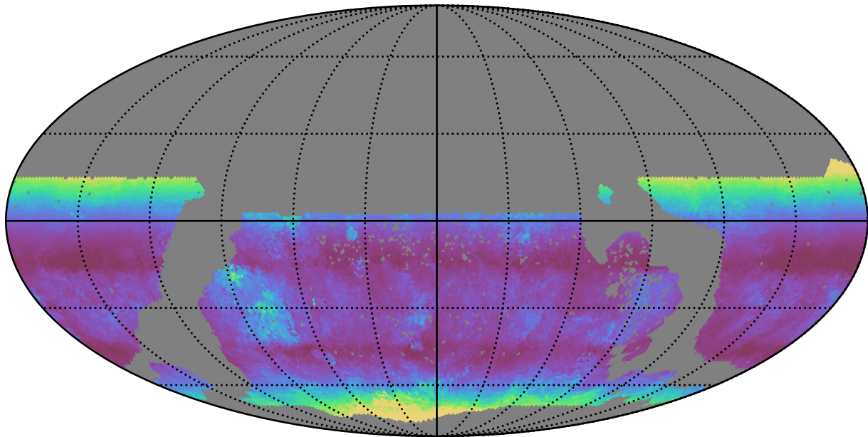
too_elab_r16_d2_gz_v3.4_10yrs WFD g band: Median airmass
