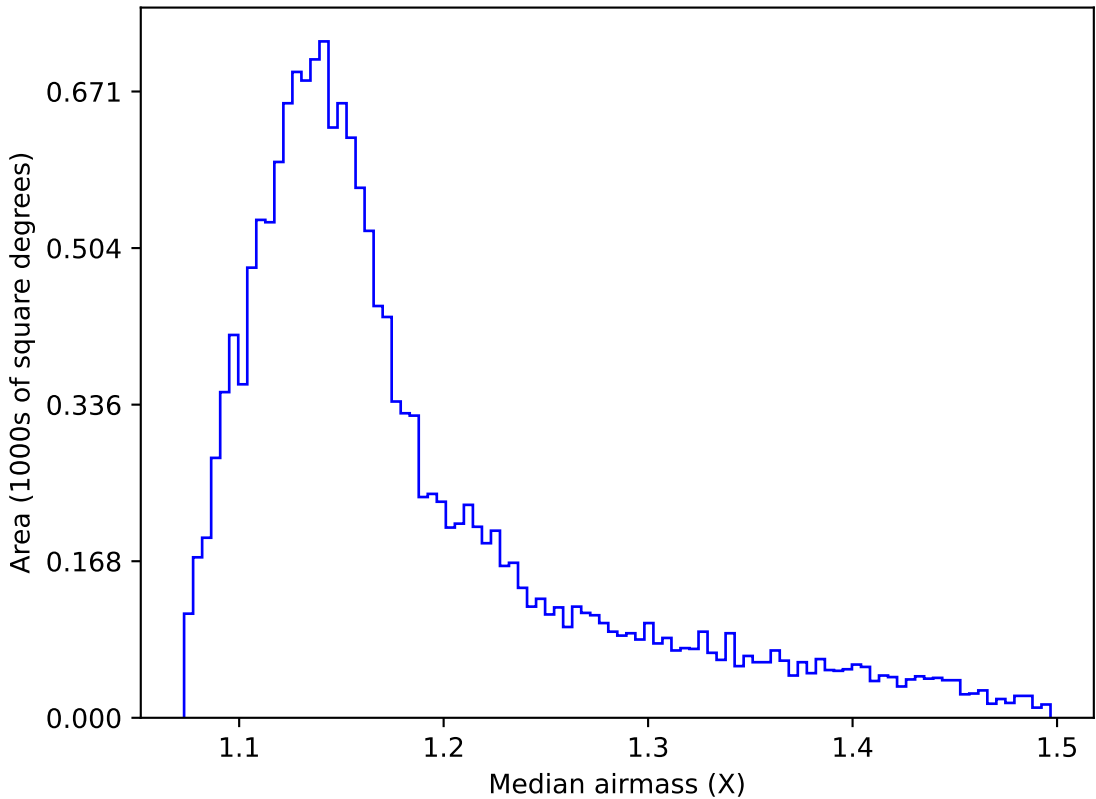
too_elab_r16_d2_gz_v3.4_10yrs WFD g band: Median airmass
