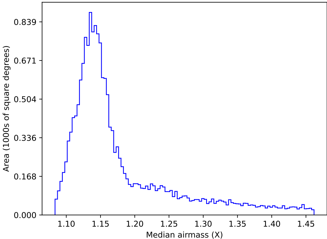
too_elab_r16_d2_gz_v3.4_10yrs WFD all bands: Median airmass
