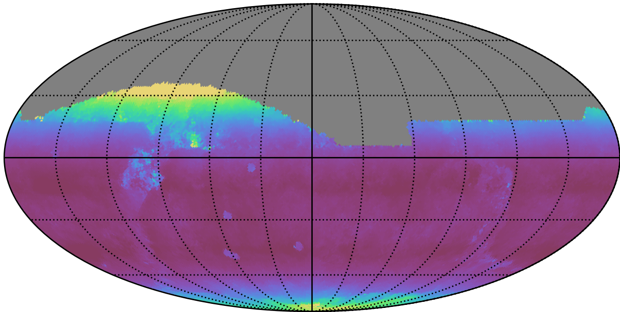
too_elab_r16_d2_gz_v3.4_10yrs All sky z band: Median airmass
