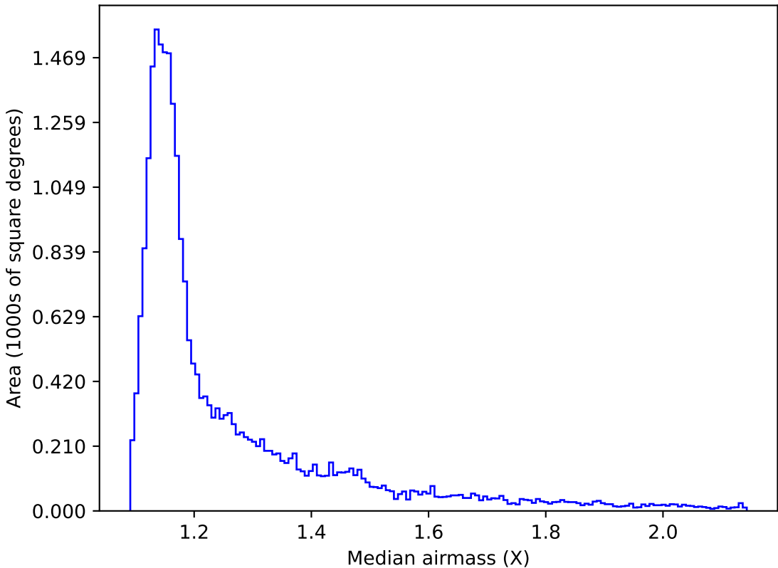
too_elab_r16_d2_gz_v3.4_10yrs All sky z band: Median airmass
